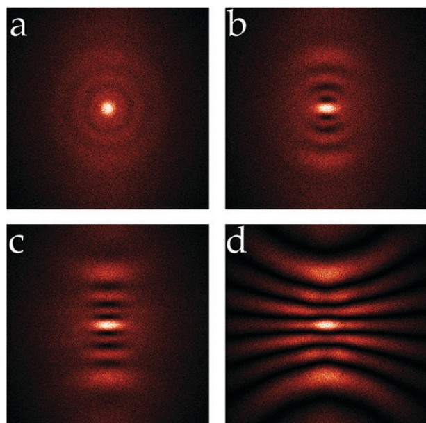
Fig. 7 Diffraction imaging patterns for 1D aligned ensembles of 2,5-diiodobenzonitrile at a X-ray energies of 8 keV (155 pm). (a) diffraction pattern of unaligned (isotropic) samples of DIBN (b)–(d) diffraction patterns of 1D aligned and oriented samples of DIBN where degrees of alignment are \theta_{\text{cl}} = 20^\circ ( \langle \cos^2\theta \rangle = 0.88 ), \theta_{\text{cl}} = 10^\circ ( \langle \cos^2\theta \rangle = 0.97 ), and \theta_{\text{cl}} = 0^\circ (“perfect” alignment), for images b, c, and d, respectively, and the orientation is always according to an up:down ratio of 10:1. The scattering angle at the mid-point of the CCD detector edge is 2\theta = 60^\circ .
