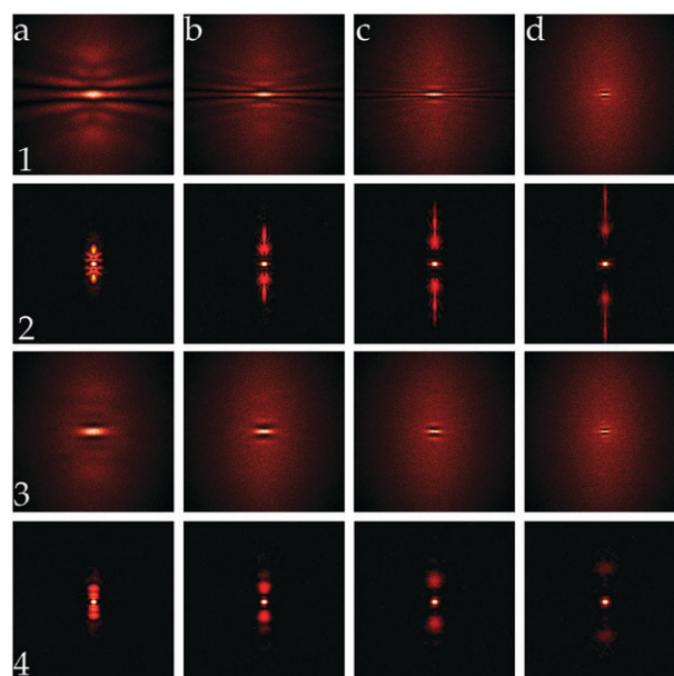
Fig. 10 Diffraction imaging patterns and their Fourier transforms for dissociating 1D aligned ensembles of 2,5-diiodobenzonitrile at an X-ray energy of 8 keV (155 pm) for pump–probe delays of (a) 0 fs, (b) 250 fs, (c) 500 fs, and (d) 1 ps. Row 1 shows the diffraction patterns of perfectly aligned samples, and row 2 the corresponding Fourier transforms. Row 3 and 4 show the same images for alignment to a cone of \pm 10^\circ .
