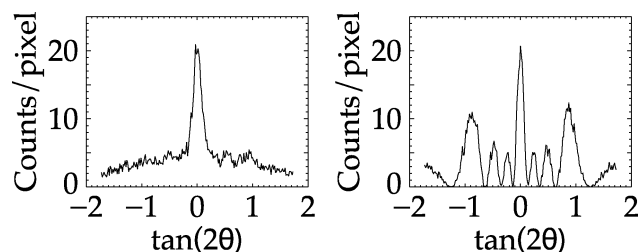
Fig. 8 Vertical lineouts of the simulated diffraction pattern of (a) unaligned and (b) 1D-aligned DIBN obtained from the images in Fig. 7 (a, d), averaged over a five pixel wide column.
