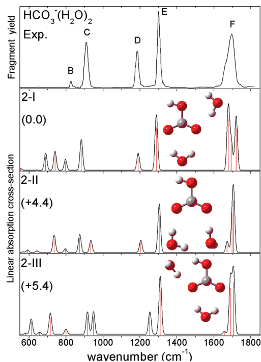
Figure 4. Experimental IRMPD spectrum of \text{HCO}_3^-(\text{H}_2\text{O})_2 (top panel), with the simulated linear absorption spectra, structures, and relative energies (kJ/mol) of the three lowest-energy isomers.
