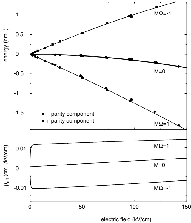
Figure 5. Measured splitting of the different M components of the CO a^3\Pi_1(v=0, J=1) A doublet as a function of the applied electric field (upper panel). The vertical axis shows the position of the energy levels relative to the centre of the A doublet in zero electric field. The full curves show the calculated Stark shift. By dividing these curves by the electric field and multiplying by -1 , the effective dipole moment is found (lower panel). (Figure reproduced from Jongma et al. (1997a) with permission. Copyright Elsevier Science.)
