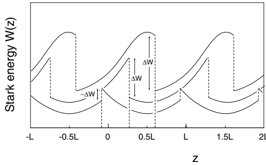
Figure 8. Potential energy for some molecules having the same velocity as the synchronous molecule ( v = L/\Delta T ). The phase of the different molecules \phi = z'\pi/L with z' the position at the moment that the fields are being switched (dashed lines) is -15^\circ , 45^\circ and 105^\circ , for the lower, middle and upper curves respectively. The different curves have been given an offset for clarity.
