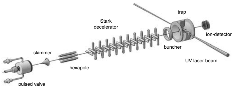
Figure 24. Schematic view of the experimental set-up. From left to right: a gas pulse of less than 1% \text{ND}_3 in Xe exits a cooled ( T = 200\text{ K} ) pulsed valve with a mean velocity of 275\text{ m s}^{-1} . The beam is focused into the decelerator and slowed down to 15\text{ m s}^{-1} . Using a ring electrode the molecules are focused (in all three directions) into a quadrupole trap. In order to detect the ammonia molecules a pulsed laser is focused inside the trap. The resulting ions are extracted and counted using an ion detector. (Figure reproduced from Bethlem et al. (2002b) with permission. Copyright the American Physical Society.)
