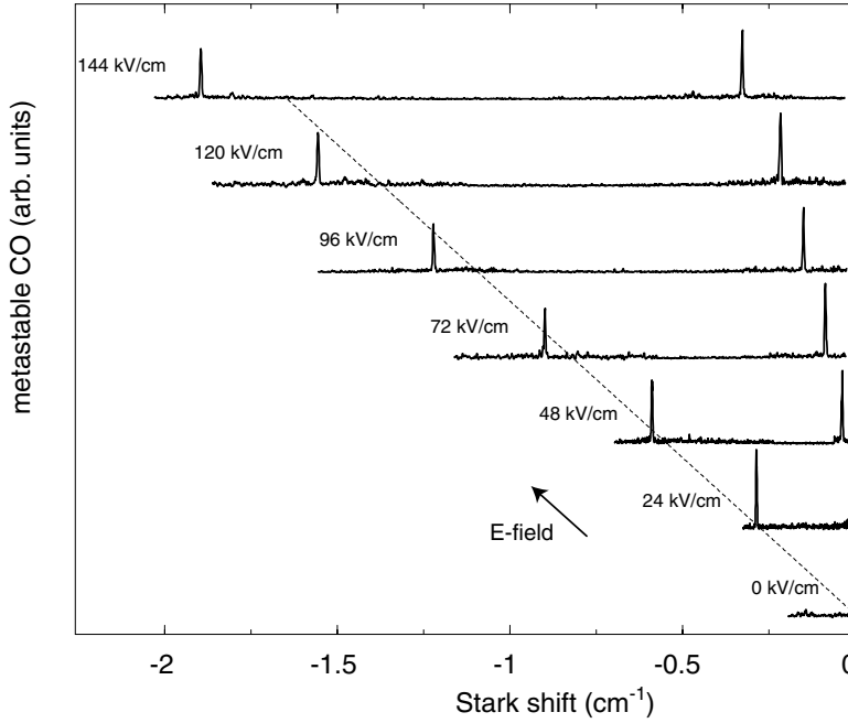
Figure 4. Excitation spectra recorded for the lower A doublet component of the a^3\Pi_1 ( v = 0 , J = 1 ) level for several values of the electric field. The horizontal axis shows the shift of the M = 0 and M\Omega = 1 level relative to the position of these levels in zero electric field. The broken line shows the calculated first-order Stark effect for the M\Omega = 1 level. (Figure reproduced from Jongma (1997) with permission.)
