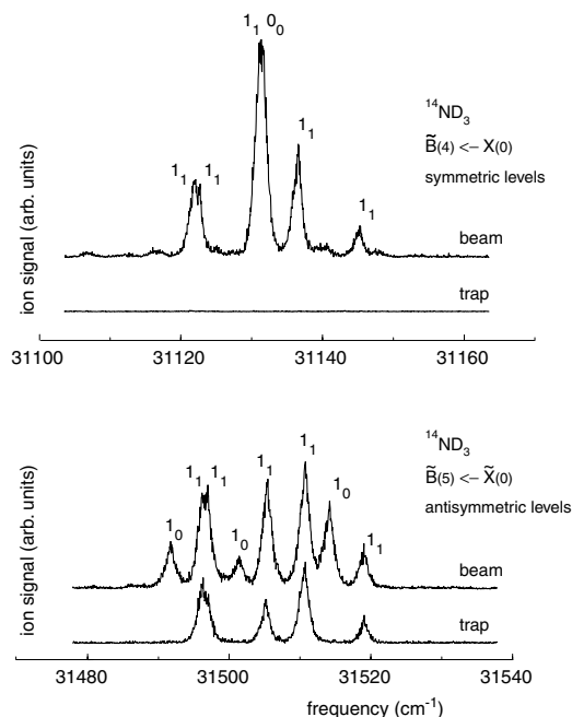
Figure 26. (2 + 1)-REMPI spectra recorded via the \tilde{B}^1E'' , \nu'_2 = 4 (upper panel) and \nu'_2 = 5 (lower panel) state in ^{14}\text{ND}_3 . In each panel, the upper curves are from measurements on the molecular beam, whereas the lower curves are recorded on the trapped molecules. (Figure reproduced from Bethlem et al. (2002b) with permission. Copyright the American Physical Society.)
