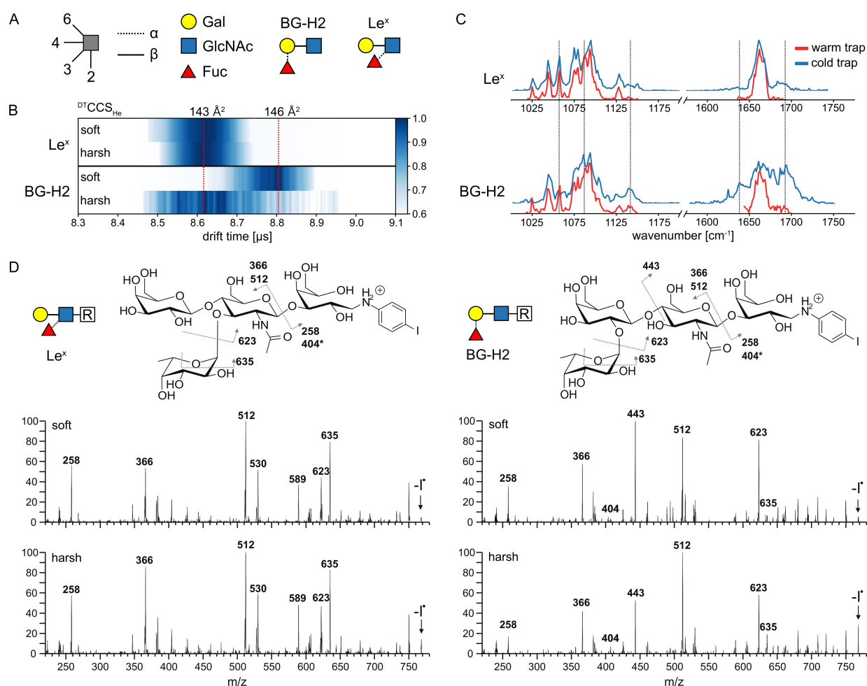
Figure 1. A) BG-H2 and \text{Le}^x trisaccharides represented using symbol nomenclature for glycans (SNFG). B) Arrival time distribution of activated (harsh conditions, 190 V cm -1 ) and non-activated (soft conditions, 30 V cm -1 ) intact precursor standards of [\text{Le}^x+\text{H}]^+ and [\text{BG-H2}+\text{H}]^+ in the heatmap representation. Upon activation, \text{DTCCS}_{\text{He}} of the [\text{BG-H2}+\text{H}]^+ ion decreases from 146 \text{\AA}^2 to 143 \text{\AA}^2 , but \text{DTCCS}_{\text{He}} of [\text{Le}^x+\text{H}]^+ of 143 \text{\AA}^2 remains unchanged. C) IR spectra of the intact [\text{Le}^x+\text{H}]^+ and [\text{BG-H2}+\text{H}]^+ standards recorded using warm (room temperature) or cold (cooled to approx. 90 K) ion trap. The spectrum of [\text{Le}^x+\text{H}]^+ remains unchanged, but the spectrum of [\text{BG-H2}+\text{H}]^+ changes (guided by dashed lines) when the temperature of the trap is changed. D) Radical fragmentation spectra afforded by photodissociation of the precursor m/z 895 and RDD of the generated radical glycan m/z 768 (indicated with an arrow). The spectra of the BG-H2-based tetrasaccharide show more pronounced differences between soft and harsh conditions compared to the spectra of the \text{Le}^x -based tetrasaccharide.
