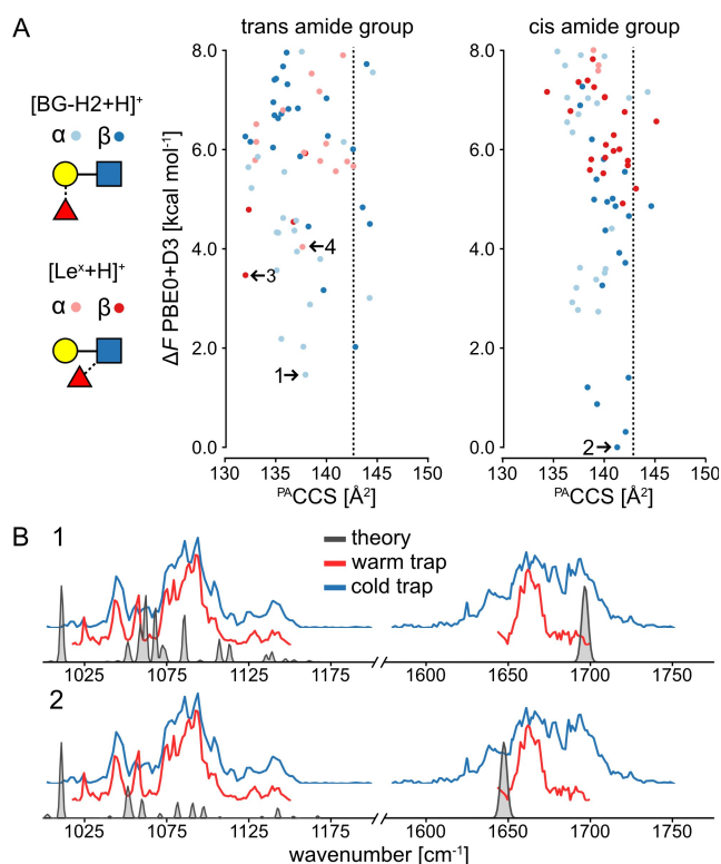
Figure 2. A) The ^{\text{PA}}\text{CCS} vs relative free energy ( \Delta F ) of conformers of the [\text{Le}^x + \text{H}]^+ and [\text{BG-H2+H}]^+ at PBE0+D3/6-311+G(d,p) level of theory. The dashed line indicates the experimental CCS, and the free energies are plotted relative to the lowest-free energy conformer of [\beta\text{-c-BG-H2+H}]^+ . The most stable anomers of each ion are highlighted. B) The comparison of the experimental and vibrational spectrum of the most stable anomers of [\text{BG-H2+H}]^+ . The comparison of the experimental and vibrational spectrum of the most stable anomers of [\text{Le}^x + \text{H}]^+ is shown in Figure S4.
