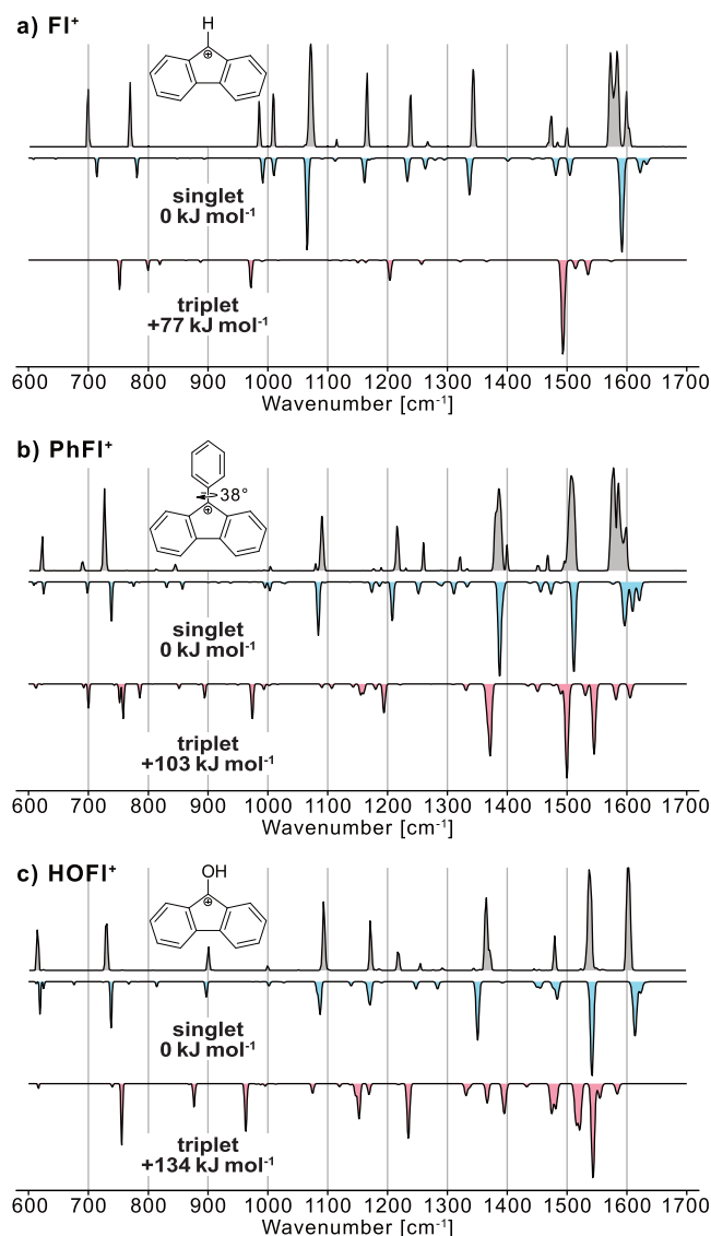
Figure 2. Infrared spectra of (a) the 9-fluorenyl cation FI + , (b) the 9-phenylfluorenyl cation PhFI + , and (c) the 9-hydroxyfluorenyl cation HOFI + . Experimental cryogenic gas-phase infrared spectra are shown as gray traces. Computed spectra for the singlet (blue) and triplet states (red) are shown in the inverted traces and originate from harmonic frequency calculations at the CAM-B3LYP+D3/def2-TZVPP level of theory. The structure and relative energies are indicated.
